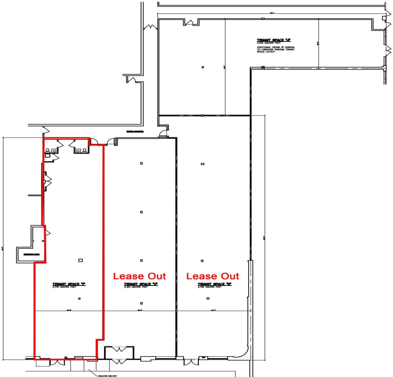
2 SK1 PROPOSED FLOOR PLAN - OPTION 2
